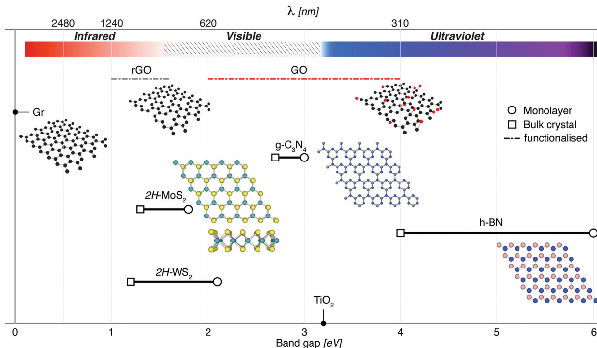
Fig. 4 2D materials which have been a focus for photocatalysis research include g-C 3 N 4 , transition metal dichalcogenides such as MoS 2 , insulators such as h-BN for composites, and other graphene-related materials (Gr, rGO and GO). Apart from graphene, which has a zero band gap, these materials can be exfoliated from their bulk materials to engineer nanosheets with a direct band gap. In the case of rGO and GO, modifications to the band gap are made possible by removing/adding functional groups. TiO 2 has been included for reference, illustrating the advantages of narrow band gap nanosheets that can target visible wavelengths for solar-driven photocatalysis. For g-C 3 N 4 , a triazine structure is shown inset. This material also has a heptazine structure which is shown in Fig. 8.
