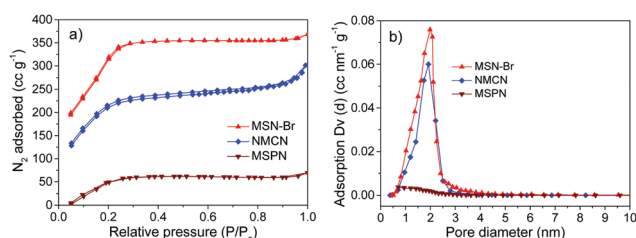
Fig. 2 (a) N 2 adsorption-desorption isotherm and (b) pore size distribution of porous MSN-Br, MSPN and NMCN nanomaterials.
