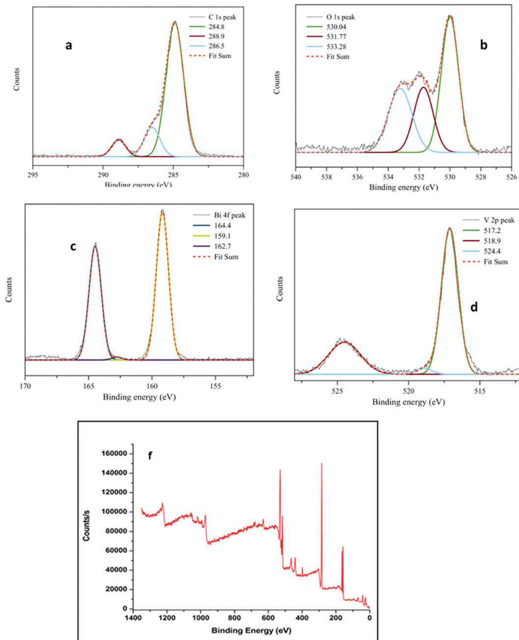
Fig. 5 High resolution XPS spectra of \text{BiVO}_4 (a) C 1s, (b) O 1s, (c) Bi 4f, (d) V 2p and (f) survey spectra.
