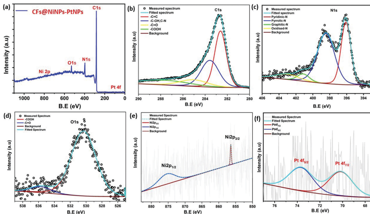
Fig. 6 (a) XPS survey spectrum of the co-axial CF@NiNP–PtNP based nanosystem and high resolution XPS spectrum of (b) C1s, (c) N1s, (d) O1s, (e) Ni2p and (f) Pt4f of the co-axial CF@NiNP–PtNP based nanosystem.
