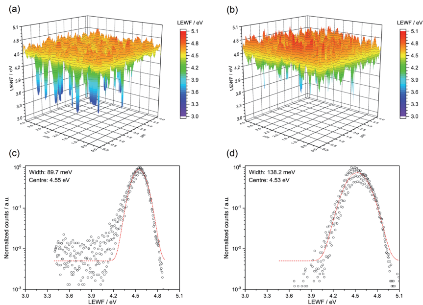
Fig. 8 LEWF maps showing the electronic terrain for (a) CZTSSe and (b) Ge5:CZTSSe after a 500 eV Ar + plasma etching treatment. Affiliated LEWF distribution showing the spread of points for (c) CZTSSe and (d) Ge5:CZTSSe.
