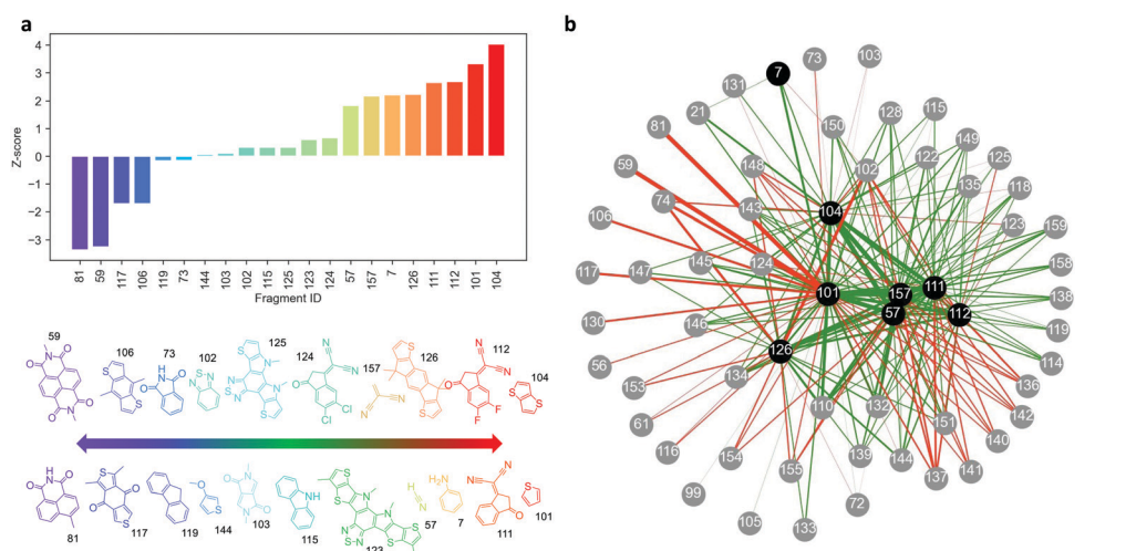
Fig. 3 (a) Z-scores obtained from the discrete hypergeometric distribution of moieties in the highly-absorbing molecules ( f_{osc,max} > 2.5 ) with respect to the entire molecular dataset, for moieties activated at least 10 times. The corresponding structures of identified moieties are shown. (b) Network graph of Z-scores relating pairs of moieties. Source nodes are coloured in black whereas child nodes are coloured in grey. The colour of the edges corresponds to the sign of the Z-score (green for positive, red for negative). The width of the edges scales with the absolute value of the Z-score.
