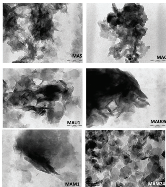
Fig. 4 TEM images (scale bar 0.1 \mu\text{m} ) for MAS, MAC MAU30, MAU60, MAM60 and MAM24.
