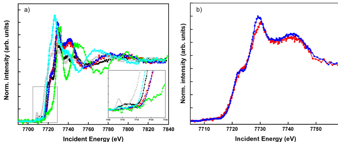
Fig. 4 (a) Co K-edge HERFD-XAS spectra of reference Co compounds along with Co(bpy) 3 2+/3+ and aged sample. (b) A comparison between fresh Co(bpy) 3 3+ /TBP and aged Co(bpy) 3 3+ /TBP samples, showing a small difference in the chemical state and reordering of ligands. The used samples were CoO, gray line; LiCoO 2 , black line; low spin Co(bpy) 3 2+ , green line; high spin Co(bpy) 3 2+ , cyan; freshly prepared Co(bpy) 3 3+ /TBP, blue; aged Co(bpy) 3 3+ /TBP, red line.
