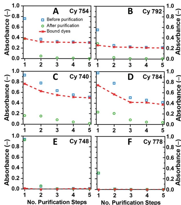
Fig. 2 Absorption peak intensity variations for MeOH solutions of NaGdF 4 :Yb,Er UCNs with Cy 754 (A), Cy 792 (B), Cy 740 (C), Cy 784 (D), Cy 748 (E), and Cy 778 (F) dyes. The initial dye concentrations are similar in all the experiments (3 \mu\text{g ml}^{-1} ). The blue square symbols show the absorption intensities of MeOH solutions before each purification step, which contain both bound and unbound dyes. The green circle symbols are related to the absorption intensities of the supernatant solutions that contain the unbound dyes. The red dashed curves are obtained by subtraction of the green from the blue values and show the absorption caused by the bound dyes.
