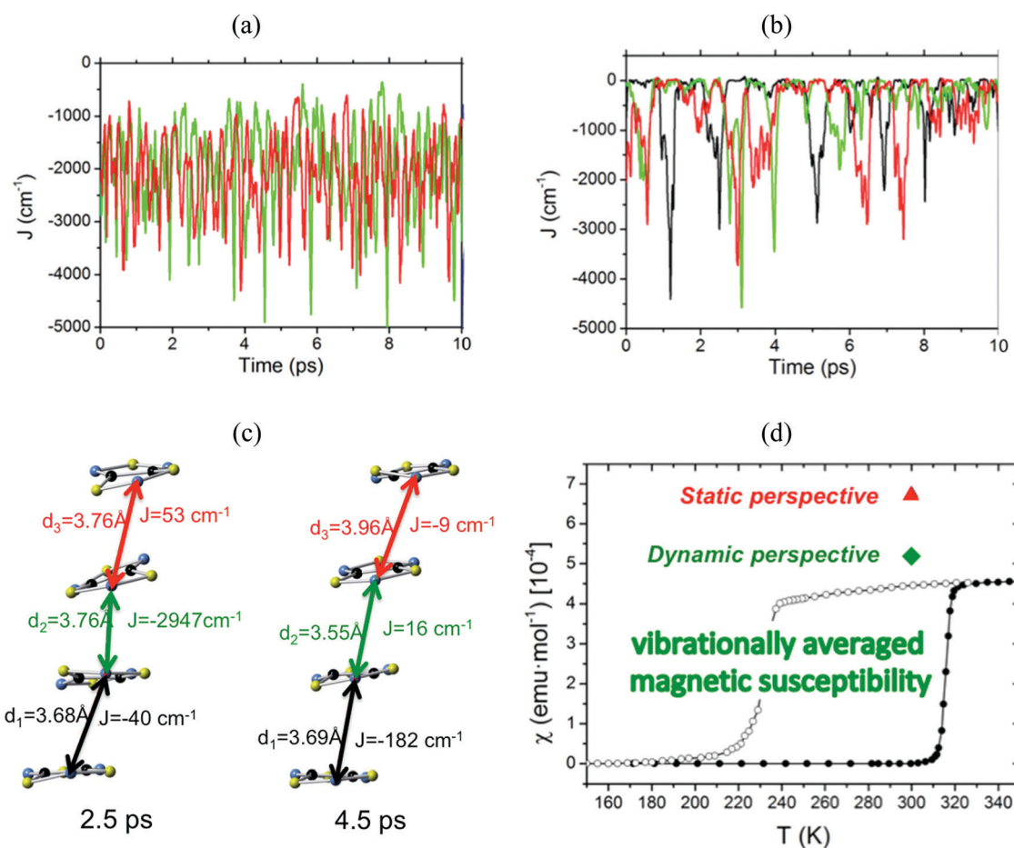
Fig. 8 Time-resolved fluctuations of (a) J(d_1) and J(d_3) for the LT polymorph, and (b) J(d_1) , J(d_2) and J(d_3) for the HT polymorph. Each of these J(d_i) values corresponds to the pair of radicals marked with d_i in Fig. 7. (c) J_{AB} values and corresponding distances in two random snapshots at 2.5 and 4.5 ps. (d) Comparison between the values of the magnetic susceptibility calculated using the static FPBU approach (red) and its vibrationally averaged counterpart (green) at 300 K. Notice that the experimental temperature dependence of the magnetic susceptibility for TTTA on cooling (empty symbols) and on heating (full symbols) is given as a reference.
