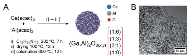
Fig. 1 (A) Synthesis of (\text{Ga},\text{Al})_2\text{O}_{3(x:y)} catalysts, where the x:y index indicates the nominal Ga : Al molar ratio used for the synthesis (1 : 6, 1 : 3, 3 : 1, 1 : 0). (B) A representative TEM image of as-prepared (\text{Ga},\text{Al})_2\text{O}_{3(1:3)} nanoparticles in toluene colloidal solution.
