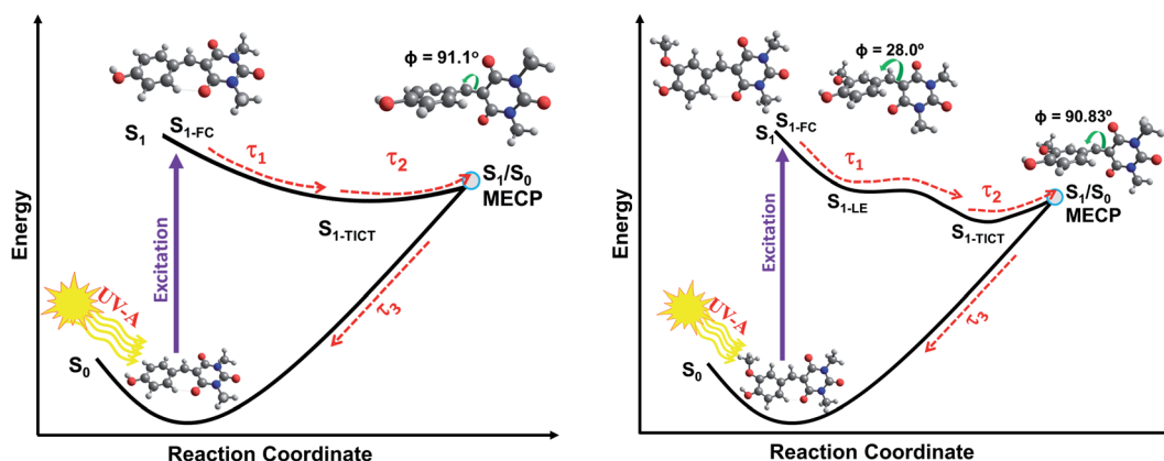
Fig. 5 Schematic of the relaxation pathways for CDDBA (left) and FDDBA- anti (right) representing the coumaryl and ferulyl series, respectively. Molecular conformations at the Franck–Condon (FC) region, at the local S_{1-LE} minimum (only for FDDBA- anti ) and at S_1/S_0 MECP are shown. The respective \phi (C1–C2–C3–C4) dihedral angles, (see Scheme 1 for atom numbering), are also indicated. The molecular structures for the S_{1-TICT} configurations are omitted here for clarity but are shown in ESI Fig. S43 and S44† and are very similar to the respective S_1/S_0 MECP geometries.
