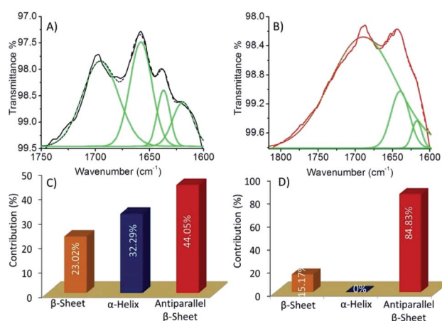
Fig. 6 (A) and (B) the FT-IR spectra of HSNPc and peptide linked 1,8-naphthalimide(control) in the amide I region ranging from 1600 to 1750 cm -1 were fitted to multiple Gaussian peaks. Deconvoluted spectra indicate each type of secondary structural component such as \alpha -helix, \beta -sheets, anti-parallel \beta -sheets and random coil. (C) and (D) Contribution (%) of each secondary structure to the self-assembled fibre network of HSNPc and control molecules that clearly shows the differences in secondary structures and hence the morphologies.
