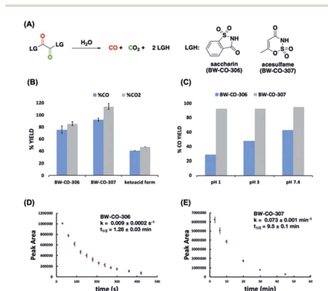
Fig. 4 (A) Structures of CO prodrugs. (B) GC-TCD analysis of CO and CO 2 yields of CO prodrugs in 4 : 1 ACN : H 2 O at 37 °C, 1 h incubation time. (C) Effect of pH on CO and CO 2 yields in 4 : 1 ACN : buffer (pH 1 – glycine/NaCl/HCl, pH 3 – citric acid/NaOH/HCl, pH 7.4 – phosphate buffer) at 37 °C, 1 h incubation time. (D) and (E) Decomposition profile of CO prodrugs in 60% PBS analyzed by RP-HPLC.
