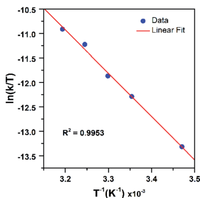
Fig. 11 Eyring plot from variable-temperature reaction kinetics of [\text{Mn}^{\text{III}}(\text{OO}^t\text{Bu})(^6\text{Me}^e\text{dpaq})]^+ with \text{PPh}_3 in \text{CH}_3\text{CN} .
