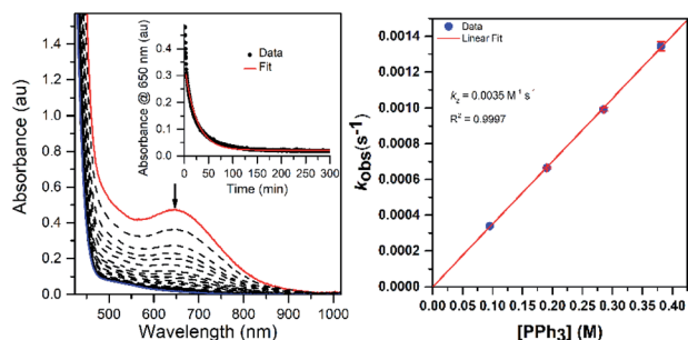
Fig. 10 Left: electronic absorption spectra monitoring the reaction of a 2.0 mM anaerobic solution of [\text{Mn}^{\text{III}}(\text{OO}^t\text{Bu})(^6\text{Me}^e\text{dpaq})]^+ (red trace) in \text{CH}_3\text{CN} with 100 equivalents of \text{PPh}_3 at 298 K. Left inset: time course for the spectral changes. Right: pseudo-first-order rate constants, k_{\text{obs}} ( \text{s}^{-1} ), versus \text{PPh}_3 concentration (M) for a 1.25 mM solution of [\text{Mn}^{\text{III}}(\text{OO}^t\text{Bu})(^6\text{Me}^e\text{dpaq})]^+ at 298 K.
