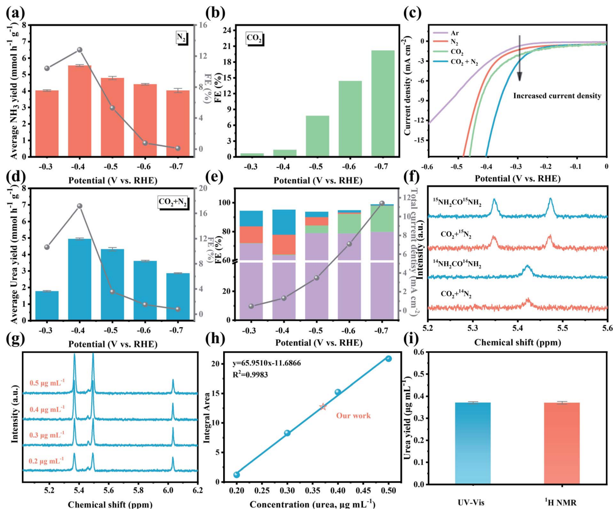
Fig. 5 (a) \text{NH}_3 synthesis with \text{N}_2 as the feed gas and (b) \text{CO} generation with \text{CO}_2 as the feed gas at various potentials for \text{BiFeO}_3/\text{BiVO}_4 hybrids; (c) LSV curves of \text{BiFeO}_3/\text{BiVO}_4 hybrids in \text{Ar} , \text{N}_2 , \text{CO}_2 and \text{N}_2 + \text{CO}_2 saturated electrolyte; (d) the urea yield rate and faradaic efficiencies and (e) the corresponding product distribution of \text{H}_2 (purple color), \text{CO} (cyan-blue color), \text{NH}_3 (red color) and urea (blue color) for urea production with \text{N}_2 and \text{CO}_2 as the feed gas at various potentials for \text{BiFeO}_3/\text{BiVO}_4 hybrids; (f) ^1\text{H} NMR spectra of electrolyte saturated with ^{15}\text{N}_2 + \text{CO}_2 , ^{14}\text{N}_2 + \text{CO}_2 after 2 h of electrolysis and standard ^{15}\text{NH}_2\text{CO}^{15}\text{NH}_2 solution; (g) ^1\text{H} NMR spectra of standard ^{15}\text{NH}_2\text{CO}^{15}\text{NH}_2 solution at concentrations of 0.2–0.5 \mu\text{g mL}^{-1} ; (h) integral area ( ^{15}\text{NH}_2\text{CO}^{15}\text{NH}_2/\text{C}_4\text{H}_4\text{O}_4 )–concentration linear relation calibrated using standard ^{15}\text{NH}_2\text{CO}^{15}\text{NH}_2 solution; (i) the urea yield of \text{BiFeO}_3/\text{BiVO}_4 hybrids after 2 h of electrolysis determined using the UV-Vis spectrum and ^1\text{H} NMR spectra.
