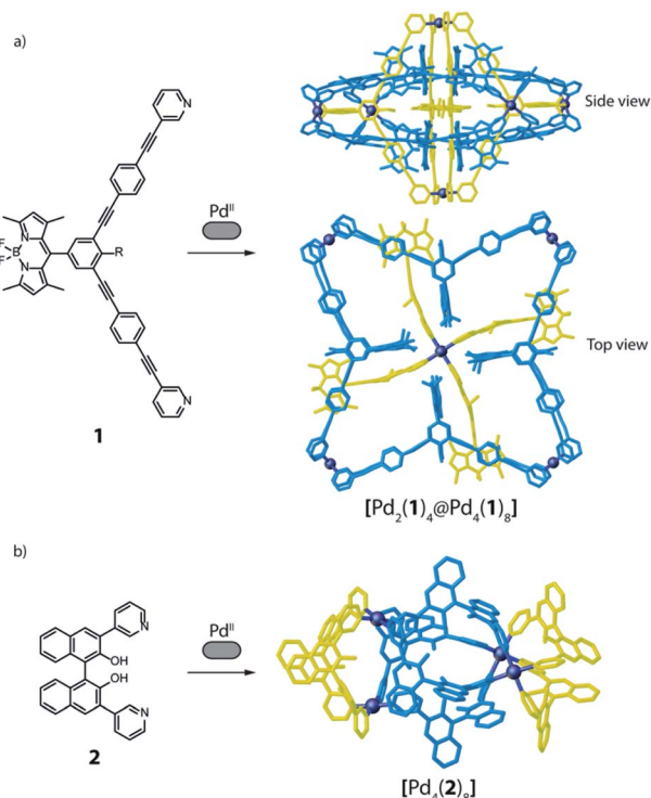
Fig. 3 (a) Ligand 1 self-assembles with Pd II cations to give a cage-in-tring architecture, where 1 occupies two different positions; (b) distorted tetrahedron obtained from a mixture of Pd II and 2 , where the ligand positions are not equivalent.
