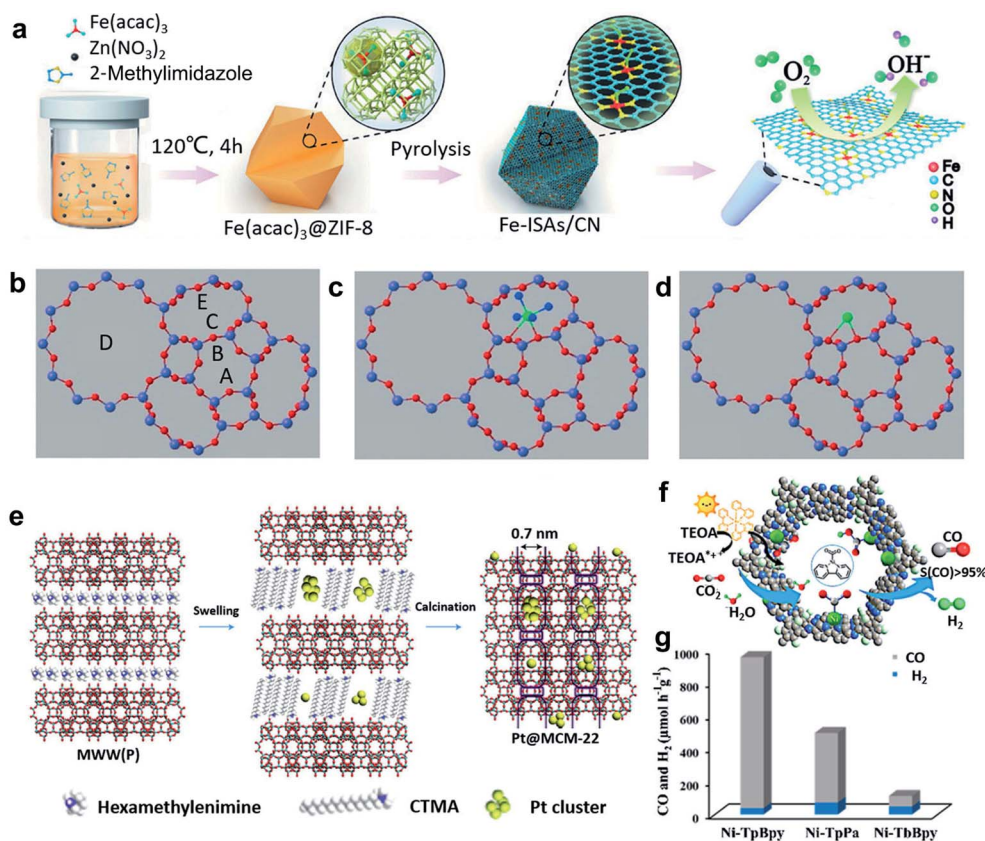
Fig. 2 (a) Schematic illustration of the formation of Fe-ISA/CN. Reproduced by permission. 22 Copyright 2017, Wiley-VCH. (b–d) Models of zeolite LTL with pore nomenclature and [Pt(NH 3 ) 4 ] 2+ and PtO x located in the 8-membered ring at the C site. Reproduced by permission. 25 Copyright 2014, Wiley-VCH. (e) Illustration of the preparation of Pt@MCM-22. Reproduced by permission. 26 Copyright 2017, Springer Nature. (f) Schematic diagram of the photocatalytic selective reduction of CO 2 over Ni-TpBpy. (g) Ni-TpBpy, Ni-TpPa, and Ni-TbBpy for the photocatalytic reduction of CO 2 in a 2 h reaction. Reproduced by permission. 28 Copyright 2019, American Chemical Society.
