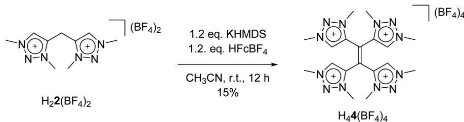
Scheme 5 Direct synthesis of \text{H}_4\text{4}(\text{BF}_4)_4 .
