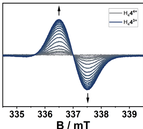
Fig. 8 EPR-spectroelectrochemical measurement of H_44^{4+} with 0.1 M NBu_4PF_6 in acetonitrile, electrolysis at -0.2 V versus silver wire at 0^\circ\text{C} .
