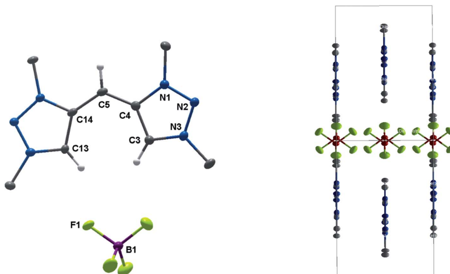
Fig. 9 ORTEP representation of [H_22^{2+}-H^+](BF_4)^- : ellipsoids drawn at 50% probability. H-atoms (except those at C3, C5 and C13) are omitted for clarity. (Left) Single molecule, (right) unit cell (for selected bond length and angles see ESI Table S4†).
