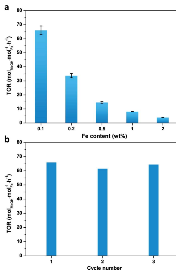
Fig. 1 (a) Turnover rate (TOR) values of various Fe/ZSM-5 catalysts with different Fe content. (b) Catalyst stability tests of methane oxidation over the 0.1% Fe/ZSM-5. (Reaction conditions: T = 50^\circ\text{C} , P_{\text{CH}_4} = 30 \text{ bar} , 0.5 \text{ M H}_2\text{O}_2 aqueous solution, catalyst mass = 0.3 g, rpm = 1500, V = 80 \text{ mL} , t = 30 \text{ min} , the deviation bar is determined from running three additional repeats.)
