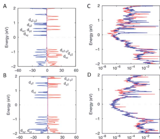
Fig. 6 Projected density of states (PDOS) of [Fe(qsal-I) 2 ] 2 NTf 2 for the high spin state (A) and low spin state (B). The projected transmission spectrum of [Fe(qsal-I) 2 ] 2 NTf 2 for the high spin state (C) and low spin state (D). Red and blue colors stand for alpha and beta spin-orbitals. The filled curves are the PDOS of the Fe III metal.
