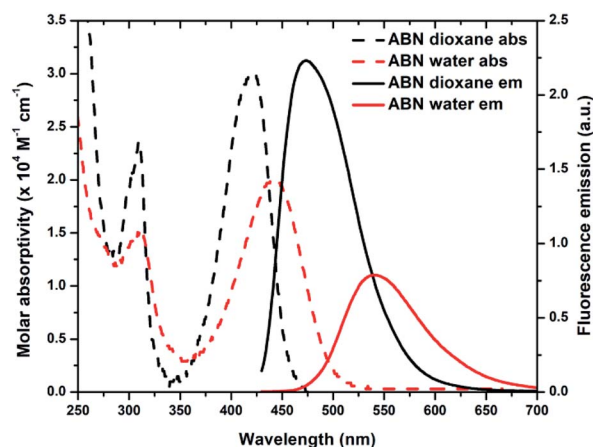
Fig. 4 Absorption (dashed line) and emission (solid line) spectra of ABN in dioxane (black) and water (red). The integral areas of emission spectra are normalized to brightness \epsilon \cdot \Phi_{em} .
