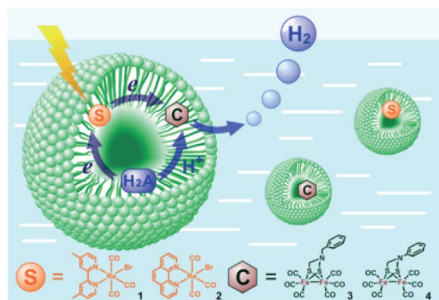
Fig. 26 A schematic representation of Re sensitizers co-embedded with [FeFe]-hydrogenase mimics in SDS micelles using ascorbic acid ( \text{H}_2\text{A} in the figure) as a sacrificial proton and electron donor. Used with permission from ref. 117.
