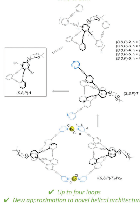
Fig. 1 Top: Previous studies with foldamers and helicene-type systems with more than two loops. Bottom: New helical systems developed in this work: chemical structure of stapled nucleus (S,S,P)-1, helical systems (S,S,P)-2–(S,S,P)-6, ligand (S,S,P)-7 and metallosupramolecular complex ((S,S,P)-7) 2 Pd 2 .
