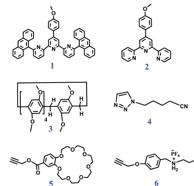
Scheme 2 Chemical structures of the model compounds 1–6 .
