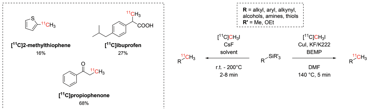
Scheme 12 The use of trialkylsilyl and trialkoxysilyl as precursors in the 11 C-methylation with [ 11 C]CH 3 I.
