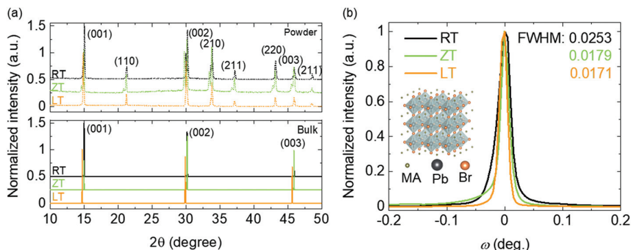
Fig. 2 X-ray diffraction of (a) powder and single crystal. (b) Rocking curve with different dissolution temperature.
