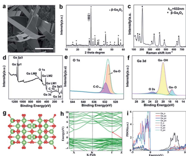
Fig. 4 Characterization of \beta\text{-Ga}_2\text{O}_3 nanobelts. (a) SEM image of hexagonal \beta\text{-Ga}_2\text{O}_3 nanobelts. (b) XRD spectrum of \beta\text{-Ga}_2\text{O}_3 . (c) Raman spectrum of the \beta\text{-Ga}_2\text{O}_3 crystal. (d–f) XPS results of \beta\text{-Ga}_2\text{O}_3 nanobelts. (g) Crystal structure of \beta\text{-Ga}_2\text{O}_3 . (h) Band structure of \beta\text{-Ga}_2\text{O}_3 . The Fermi energy is aligned to zero. (i) PDOS of \beta\text{-Ga}_2\text{O}_3 . The scale bar in (a) is 10 \mu\text{m} .
