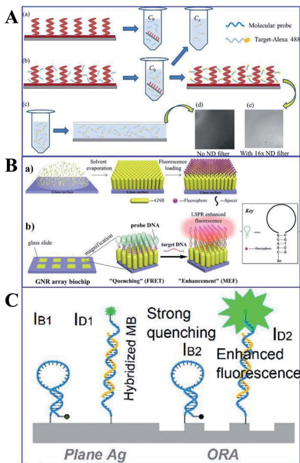
Fig. 13 (A) Schematic of the (a) molecular probe binding to AgNRs and (b) fluorophore labelled target oligonucleotide hybridizing with the molecular probe, with its fluorescence image in (e). (c) A drop of the target-alexa488 is sandwiched between the Si wafer and a piece of cover slip for fluorescence measurement, with the fluorescence image shown in (d). Reprinted from ref. 118 with permission. (B) Schematic showing (a) the fabrication processes of the ordered standing GNR, and (b) practical applications of the GNR array chip for DNA detection. Reprinted TOC figure with permission from Zhong Mei and Liang Tang, Anal. Chem. , 2017, 89 , 633–639 (ref. 100). Copyright 2017 American Chemical Society. (C) Schematic showing MBs anchored on the ORAs and plane silver surfaces respectively. IB1/IB2: quenched background intensities on plane silver/ORAs, ID1/ID2: fluorescence signals of hybridized MBs on plane silver/ORAs surfaces, respectively. Reprinted TOC figure with permission from Akash Kannegulla, Ye Liu, Bo Wu and Li-Jing Cheng, J. Phys. Chem. C , 2018, 122 , 770–776 (ref. 152). Copyright 2018 American Chemical Society.
