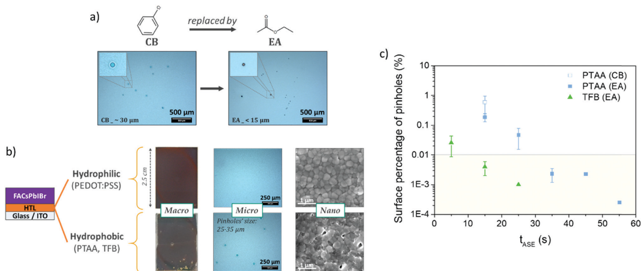
Fig. 2 (a) Impact of anti-solvent's nature (chlorobenzene vs. ethyl acetate) on the micro-scale pinholes in the perovskite layer (examples on the PTAA layer, t_{\text{ASE}} = 15 s); (b) impact of the HTL nature (hydrophilic vs. hydrophobic) on the perovskite layer at macro-, micro- and nano-scales (examples with EA, t_{\text{ASE}} = 15 s); and (c) surface pinhole proportion (determined by optical microscopy, see Fig. S3, ESI†) as a function of anti-solvent ejection time ( t_{\text{ASE}} ) and HTL nature.
