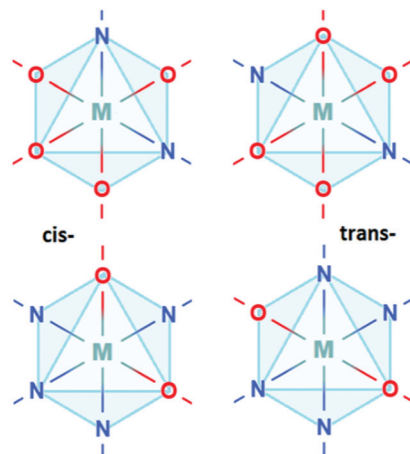
Fig. 1 Anion ordering in M-O_4N_2 and M-O_2N_4 octahedra.
