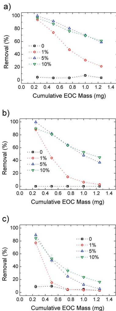
Fig. 9 Removal efficiency for Ciproflox (a), OFLOX (b) and RhB (c) for PES and increasing GO loading in HF-GO. The cumulative initial mass is obtained with fixed concentration ( 5 \text{ mg L}^{-1} ) and flow ( 15 \text{ mL min}^{-1} ). Details are reported in Fig. S10. The curves for HF-GOe filters are shown in Fig. S11, ESI†
