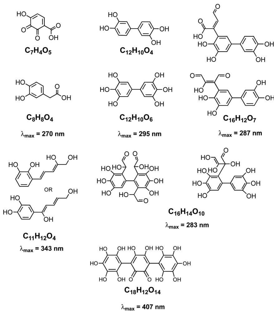
Scheme 2 Structure of molecules and oligomers and their characteristic absorption wavelength detected in the reaction of catechol with \text{Fe(III)} under conditions characteristic of viscous multicomponent aerosol systems with relatively high ionic strength ( I = 1\text{--}12 \text{ m} ) and acidic pH ( \sim 2 ) using UHPLC-MS. Modified from ref. 148 with permission from The American Chemical Society, © 2021.
