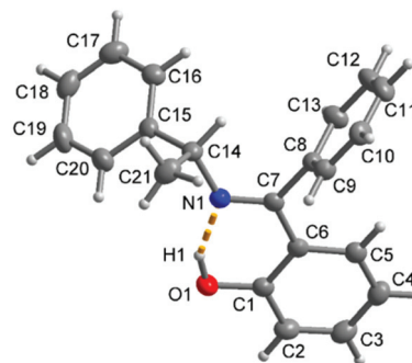
Fig. 3 Molecular structure of R\text{-HL}^1 with the dashed orange line showing the intramolecular hydrogen bond with \text{O1}\cdots\text{H1} 0.91(2) Å, \text{H1}\cdots\text{N1} 1.70(3) Å, \text{O1}\cdots\text{N1} 2.533(2) Å, \text{O1-H1}\cdots\text{N1} angle 151(2)^\circ .
