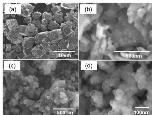
Fig. 6 Schematic illustration of the preparation of nano sized ZSM-5 zeolite crystals by ball milling and subsequent recrystallisation (top panel) and SEM images of zeolite A (LTA) crystals: pristine (a), post milling (b) and after subsequent recrystallisation (c and d). Adapted and reproduced with permission from ref. 97 Copyright (2011) American Chemical Society.
