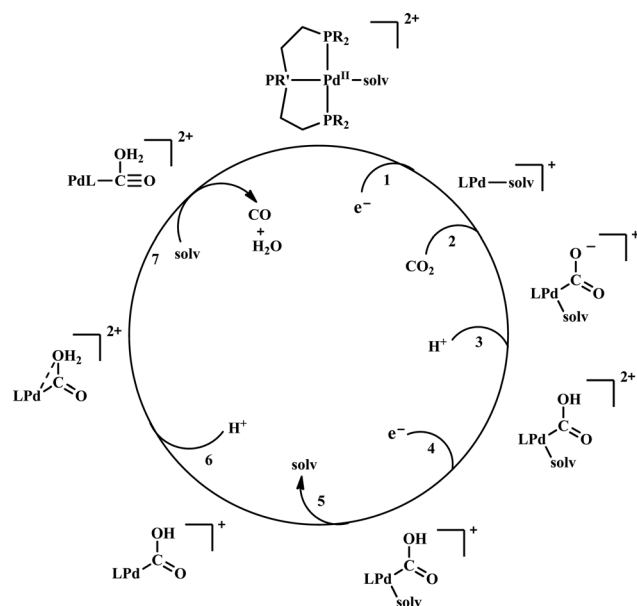
Scheme 6 General mechanistic scheme for the electrocatalytic CO 2 reduction by [Pd(triposphine)(S)] 2+ catalysts.
