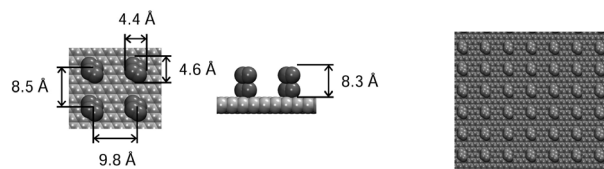
Fig. 1 Topological details (left) and top view (right) of the corrugated surface. The posts of specified dimensions are planted along lateral ( x,y ) directions on the surface, which spans the entire box in the y direction, while it is of finite width smaller than the width of the box in the x direction. The system is periodically replicated along the x and y directions.
