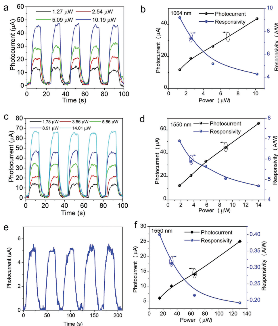
Fig. 4 (a) Time dependent photocurrent of the graphene–Mo _2 C device with a large Mo _2 C sheet tested at 1064 nm under different irradiation powers. Source–drain bias: 1 V, zero gate voltage. (b) Photocurrent and responsivity as a function of laser powers at 1064 nm for graphene–Mo _2 C device with large Mo _2 C sheet. (c) Time dependent photocurrent of the graphene–Mo _2 C device with the large Mo _2 C sheet tested at 1550 nm under different irradiation powers. Source–drain bias: 1 V, zero gate voltage. (d) Photocurrent and responsivity as a function of laser powers at 1550 nm for the graphene–Mo _2 C device with the large Mo _2 C sheet. (e) Time-dependent photocurrent of the graphene–Mo _2 C device with small Mo _2 C sheets tested at 1550 nm under the irradiation power of 15 \mu W. (f) Photocurrent and responsivity as a function of laser powers at 1550 nm for the graphene–Mo _2 C device with small Mo _2 C sheets.
