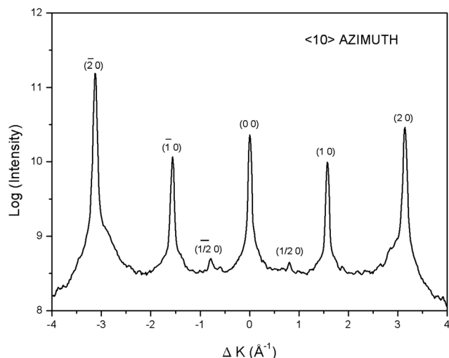
Fig. 1 Angular distribution for a 52% Nb KTN target in the \langle 10 \rangle azimuth. The intensities are plotted logarithmically to emphasize the presence of half order diffraction peaks. The surface temperature is 190 K.
