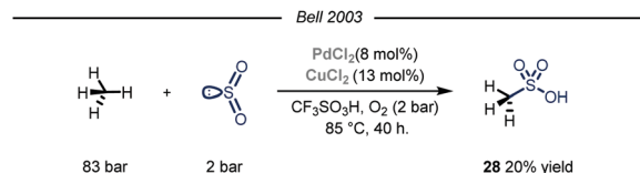
Fig. 17 \text{Pd}(\text{II}) - \text{Cu}(\text{II}) dual catalytic manifold for the conversion of methane into methanesulfonic acid.
