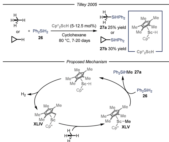
Fig. 16 Scandium-catalyzed silylation of light alkanes through C-H activation. \text{Cp}^* : pentamethylcyclopentadienyl.
