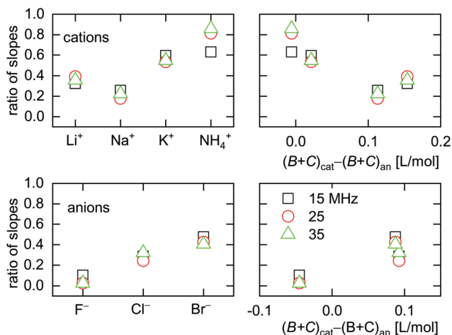
Fig. 9 Ratio of slopes \langle A/\Delta E \rangle_{\Delta f} / (-\langle A/\Delta E \rangle_{\Delta f}) as obtained from \Delta f and \Delta E (eqn (13)). Large ratios indicate a large elastic contribution. \text{Cs}^+ was omitted from this graph because the sign of \langle A/\Delta E \rangle_{\Delta f} for \text{Cs}^+ was opposite to the sign of \langle A/\Delta E \rangle_{\Delta f} for all other ions.
