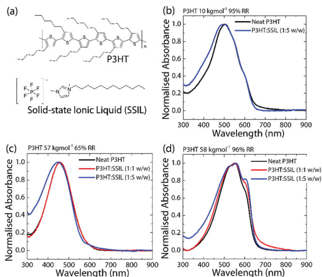
Fig. 1 (a) Chemical structure of the conjugated polymer P3HT and the solid state ionic liquid [C 12 H 25 N + ][PF 6 - ] (SSIL). Normalised absorbance spectra of P3HT neat, 1:1 and 1:5 for (b) low M_w and high RR, (c) high M_w and low RR and (d) high M_w and RR P3HT blends.
