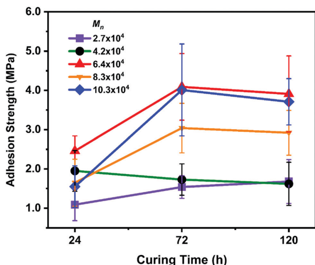
Fig. 1 Adhesion strength with different curing times. Error bars indicate standard deviation, n \geq 5 .
