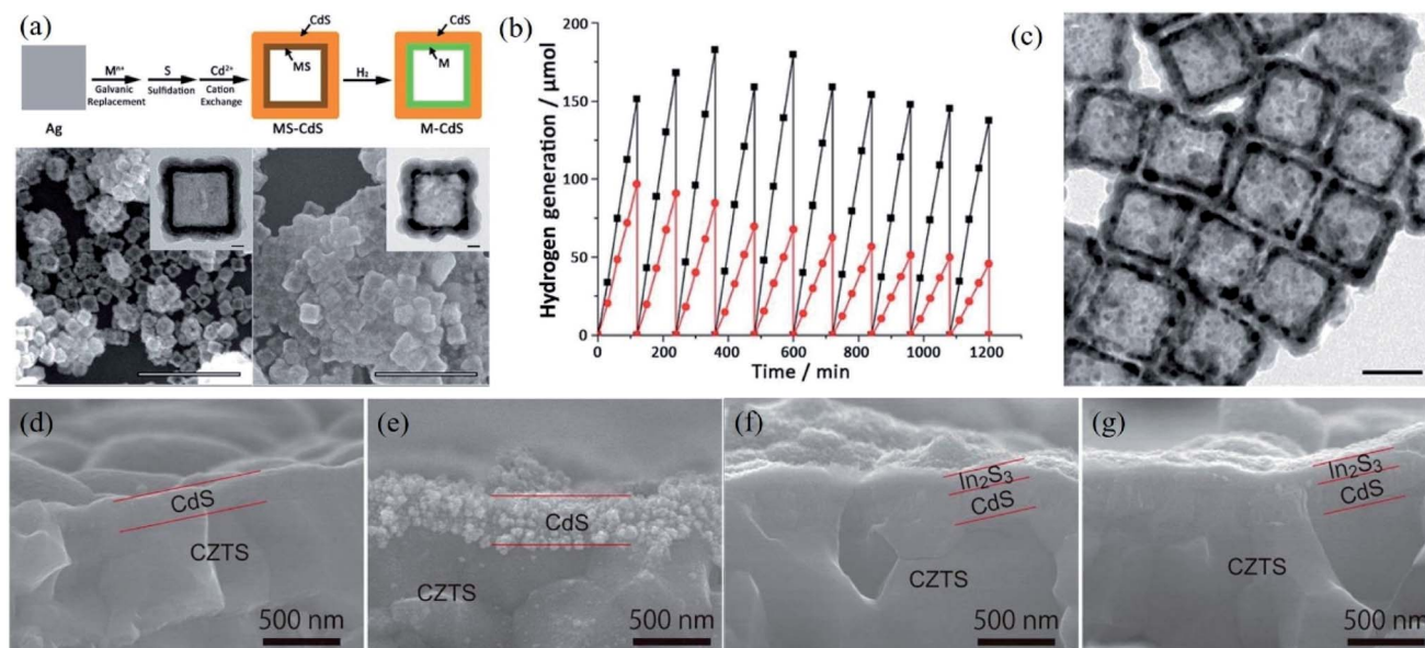
Fig. 7 (a) General synthetic approach of M–CdS double shell hollow nanocubes ( M = \frac{1}{2}\text{Pt} , Au, and Pd) and SEM and TEM images of PtS–CdS and Pt–CdS hollow nanocubes; (b) time course of \text{H}_2 generation using Pt–CdS double shell hollow nanocubes (black) and commercial CdS platinized by photo-deposition (red); (c) TEM image of Pt–CdS hollow nanocubes after 10 cycles of \text{H}_2 generation. Reprinted with permission from ref. 116. Copyright 2016, Royal Society of Chemistry. (d–g) Cross-sectional SEM images of (d, e) Pt/CdS/CZTS and (f, g) Pt/ \text{In}_2\text{S}_3 /CdS/CZTS photo-cathodes before (d, f) and after (e, g) a 3 h durability test. Reprinted with permission from ref. 117. Copyright 2015, American Chemical Society.
