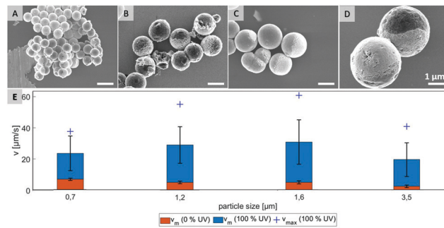
Fig. 3 SEM pictures of Janus particles with average sizes of 0.7 \mu\text{m} (A), 1.2 \mu\text{m} (B), 1.6 \mu\text{m} (C), 3.5 \mu\text{m} (D) and their velocities (E) in 0.5% H 2 O 2 solution ( v_m – mean velocity at given UV intensity, v_{\text{max}} – velocity of fastest particle), scale bar 1 \mu\text{m} .
