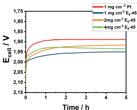
Fig. 6 Chronopotentiometry of Pt/C and \text{E}_{8-45}/\text{C} at a catalytic loading of 1–4 \text{mg cm}^{-2} at 80 ^{\circ}\text{C} for 5 h at an applied current of 1 \text{A cm}^{-2} .
