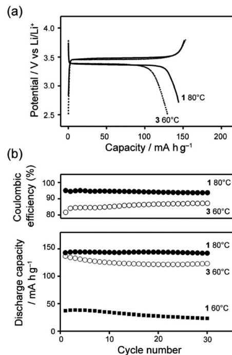
Fig. 7 (a) Comparison of representative charge–discharge curves between LC mixture of 1 and LiTFSI (black line) and LC mixture of 3 and LiTFSI (dotted line) at the 5th cycle. (b) Cyclability and coulombic efficiency of Li half-cells using LC electrolytes.
