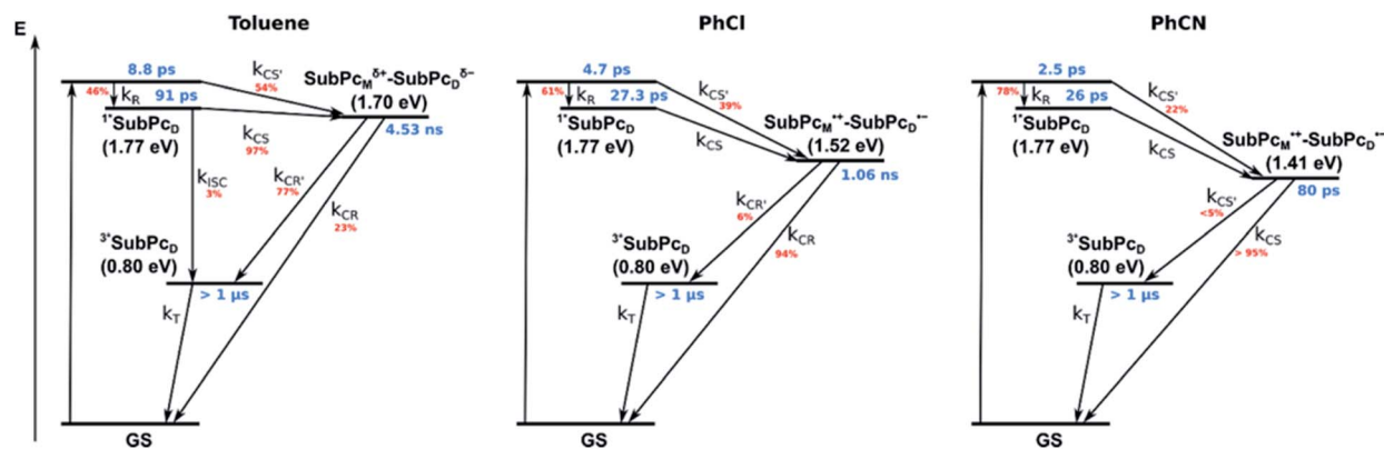
Fig. 11 Energy diagrams of syn -SubPc 1 in toluene, PhCl, and PhCN illustrating the excited state deactivation after 656 nm laser excitation at room temperature. Lifetimes and scaling parameters were obtained by global target analysis of the transient absorption data.
