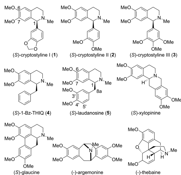
Scheme 1 Representative THIQAs.
