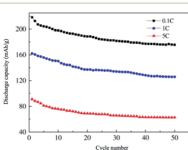
Fig. 17 Cyclic performance of nano \text{C}/\text{Li}_2\text{MnSiO}_4 synthesized by ionothermal method, the material is tested in the potential range of 2.5–4.5 V. 153
